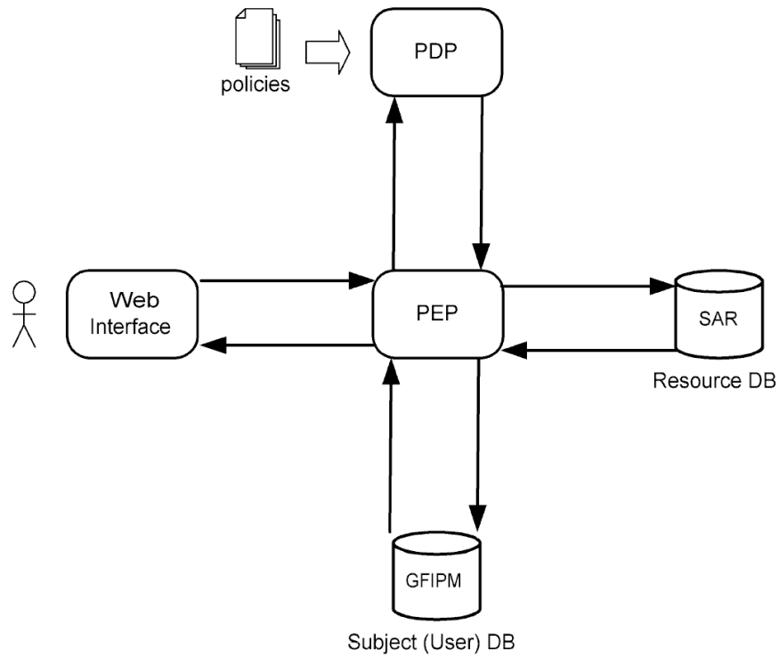
Figure 4. PET architecture.
